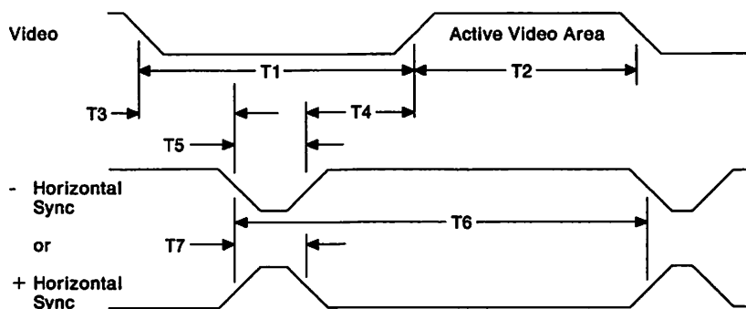
Figure 4-7. Vertical Timing, 768 Lines. Type 1 video does not support these timings.
