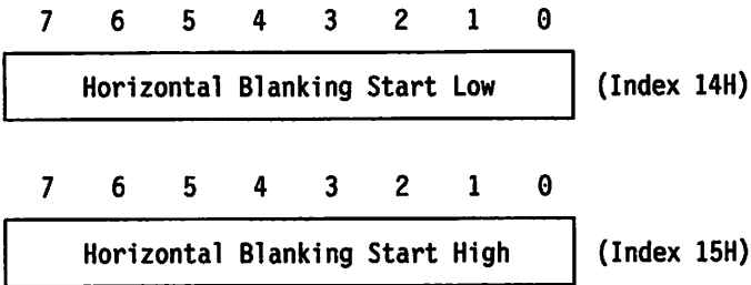
Figure 3-30. Horizontal Blanking Start Registers, Indexes Hex 14 and 15
