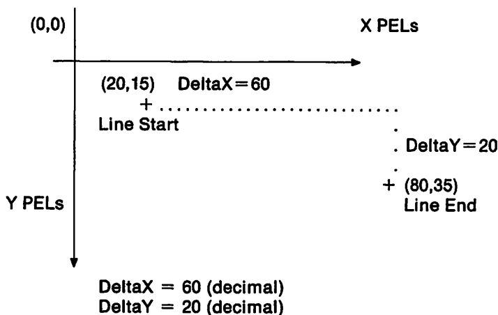
Figure 3-190. Line Draw Example in Octant 0
