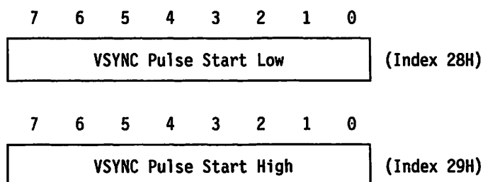
Figure 3-48. Vertical Sync Pulse Start Registers, Indexes Hex 28 and 29
