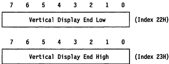
Figure 3-42. Vertical Display End Registers, Indexes Hex 22 and 23
