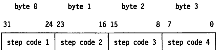
Figure 3-125. Direction Steps Register, Offset Hex 2C
