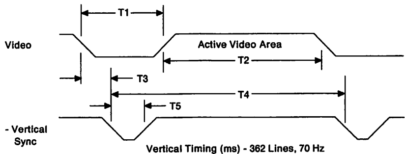
Figure 4-3. Vertical Size of Display
