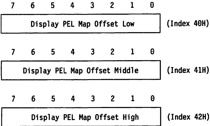
Figure 3-63. Display PEL Map Offset Registers, Indexes Hex 40 – 42
