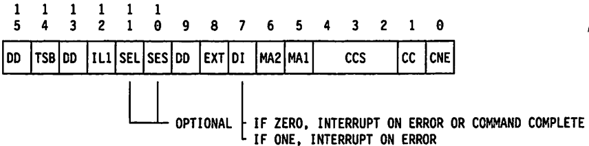
Figure 60. SCB Enable Word 1
