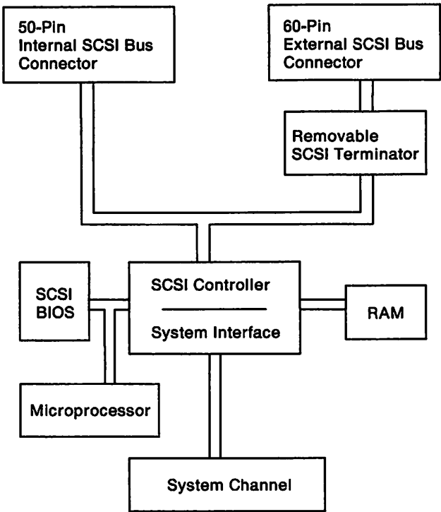
Figure 1. Subsystem Block Diagram
