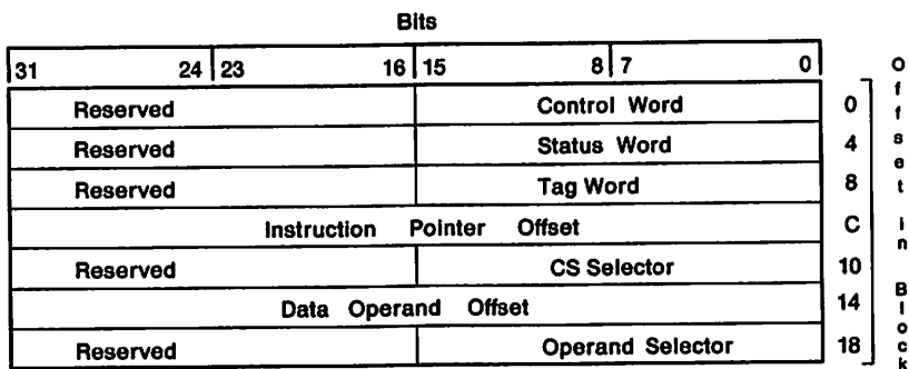
Figure 31. Instruction and Pointer Image (32-Bit Protected Mode)
