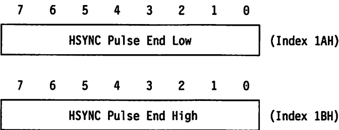
Figure 3-36. Horizontal Sync Pulse End Registers, Indexes Hex 1A and 1B
