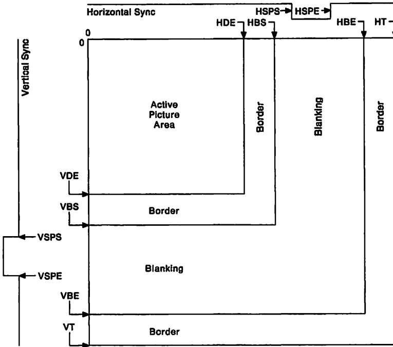
Figure 3-5. CRT Controller Register Definitions
