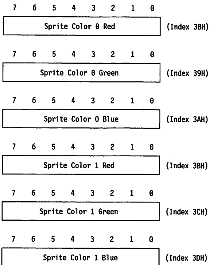
Figure 3-62. Sprite Color Registers, Indexes Hex 38 – 3D
