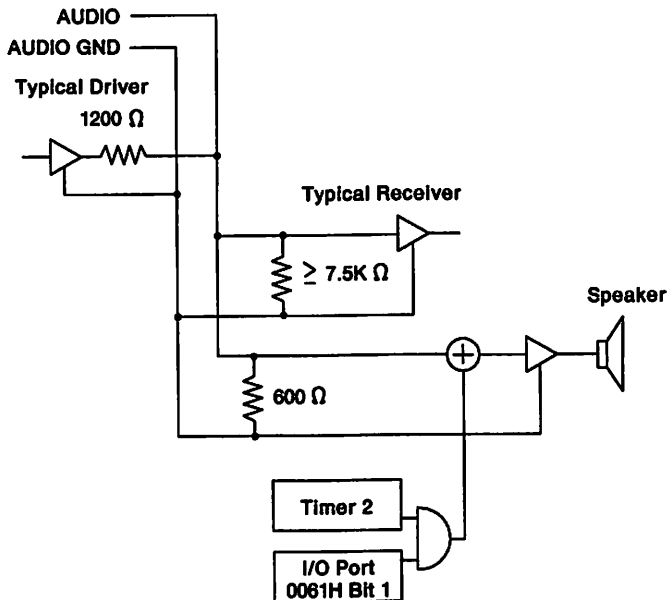
Figure 2. Audio Subsystem Block Diagram
