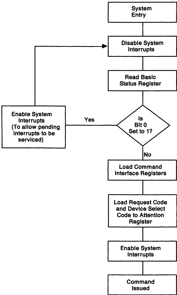
Figure 18. Issuing a Command
