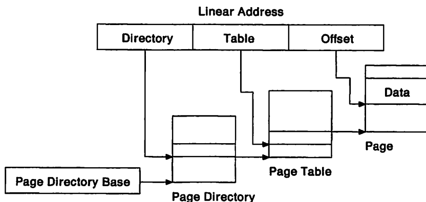
Figure 3-167. Linear to Physical Address Translation
