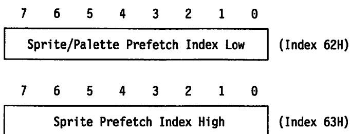
Figure 3-78. Sprite/Palette Prefetch Index Registers, Indexes 62 and 63
