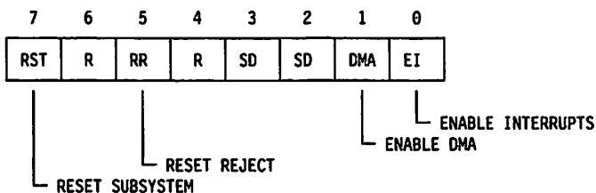
Figure 63. SCB Subsystem Control Register
