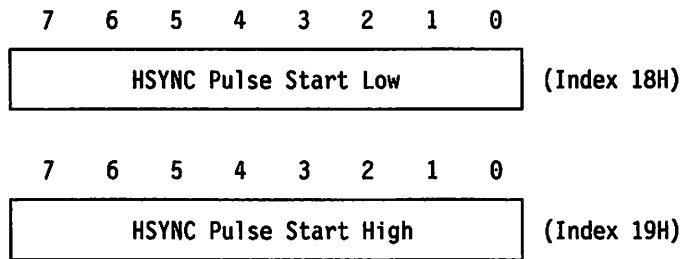
Figure 3-34. Horizontal Sync Pulse Start Registers, Indexes Hex 18 and 19
