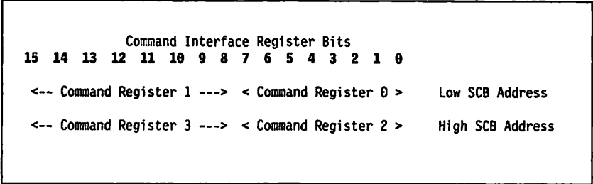
Figure 8. Register Content for SCB
