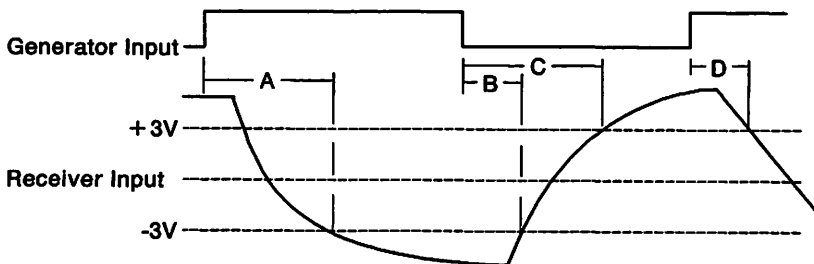
Generator Waveforms
