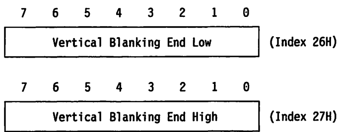
Figure 3-46. Vertical Blanking End Registers, Indexes Hex 26 and 27
