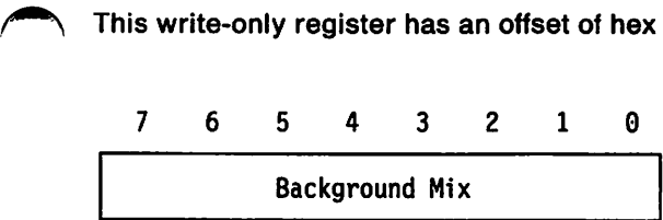
Figure 3-127. Background Mix Register, Offset Hex 49
