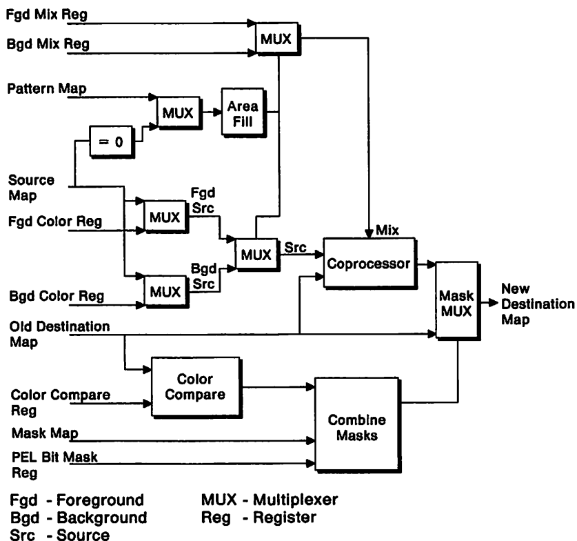
Figure 3-92. Coprocessor Data Flow
