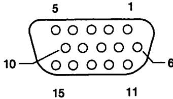
Figure 4-1. Display Connector
