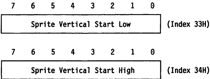
Figure 3-57. Sprite Vertical Start Registers, Indexes Hex 33 and 34
