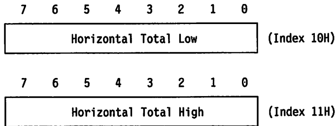
Figure 3-26. Horizontal Total Registers, Indexes Hex 10 and 11
