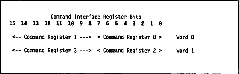
Figure 9. Register Content for Immediate Command
