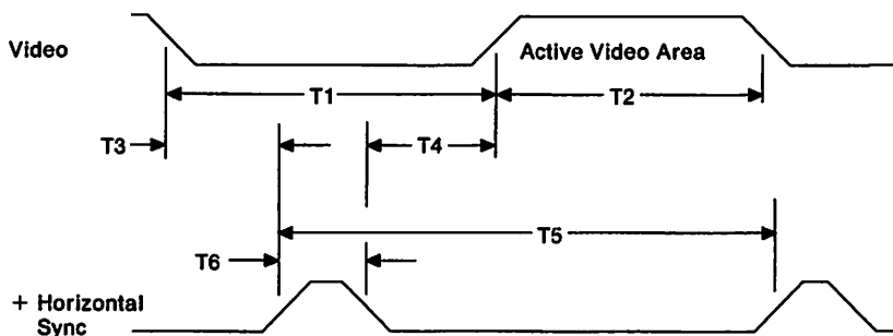
Figure 4-9. Horizontal Timing, 40/80 Column, without Border
