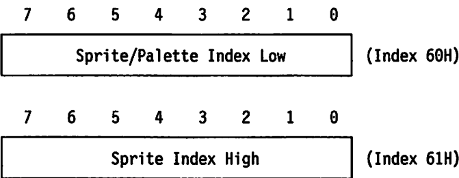
Figure 3-77. Sprite/Palette Index Registers, Indexes Hex 60 and 61
