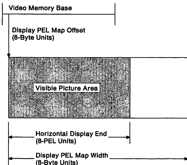
Figure 3-6. Display PEL Map Offset and Width Definitions
