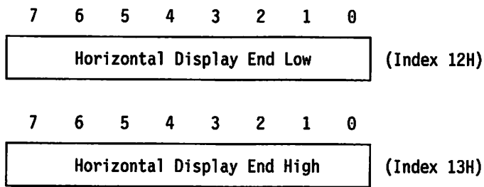
Figure 3-28. Horizontal Display End Registers, Indexes Hex 12 and 13
