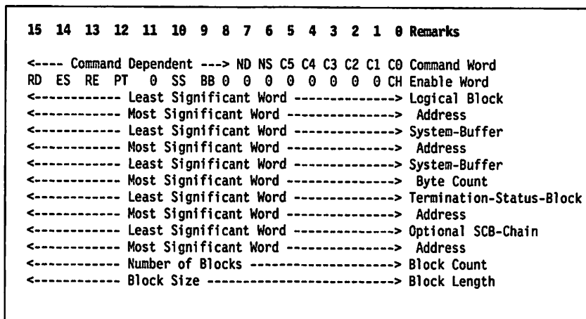
Figure 20. Subsystem Control Block Structure
