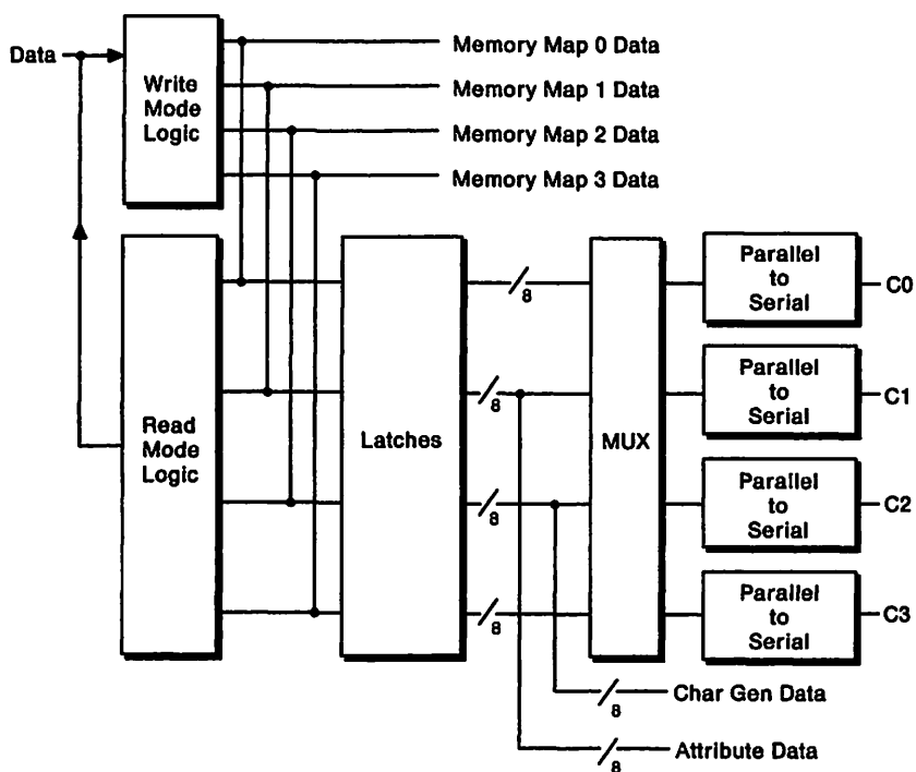
Figure 2-2. Graphics Controller
