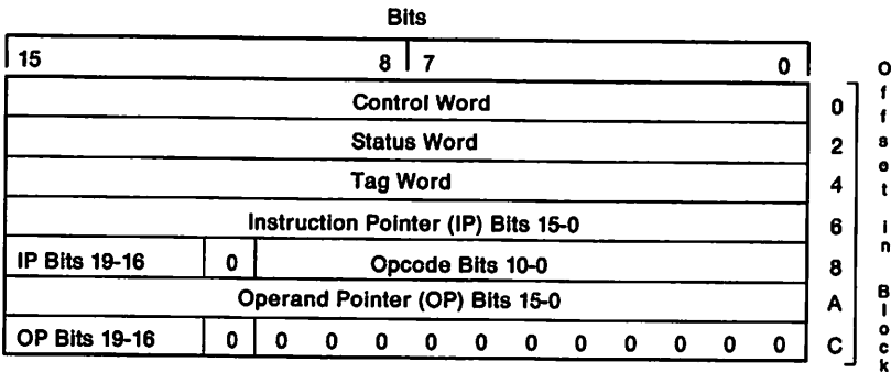
Figure 28. Instruction and Pointer Image (16-Bit Real Address Mode)
