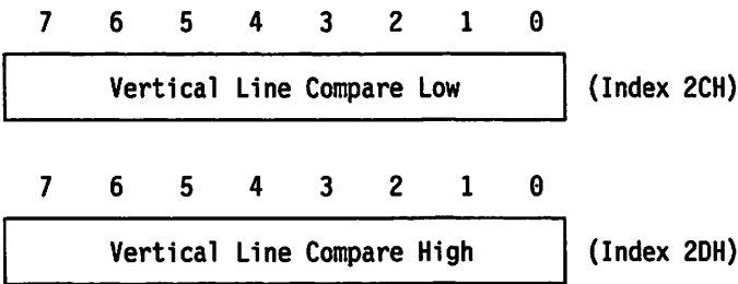
Figure 3-51. Vertical Line Compare Registers, Indexes Hex 2C and 2D
