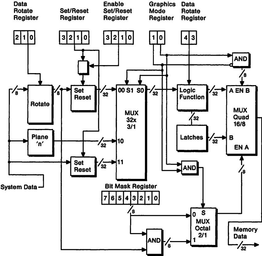
Figure 2-17. Data Flow for Write Operations
