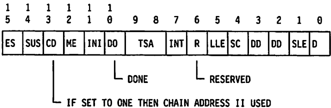
Figure 61. SCB End Status Word 1
