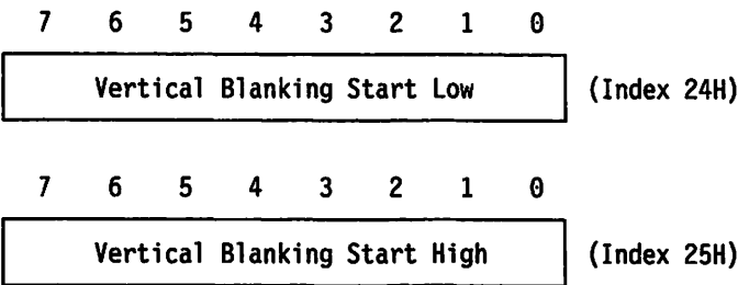
Figure 3-44. Vertical Blanking Start Registers, Indexes Hex 24 and 25
