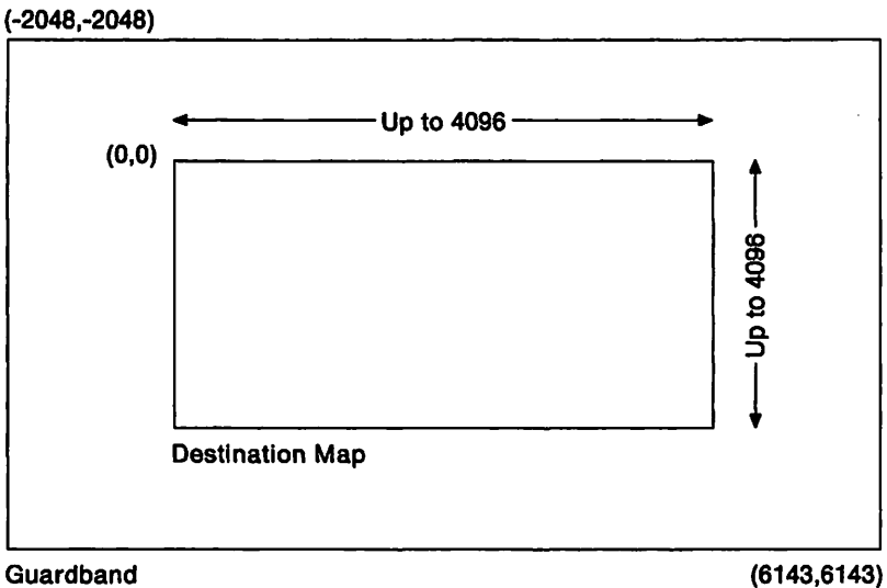
Figure 3-95. Destination Map Guardband
