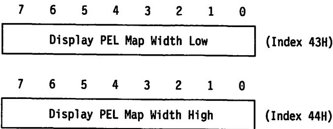
Figure 3-65. Display PEL Map Width Registers, Indexes Hex 43 and 44
