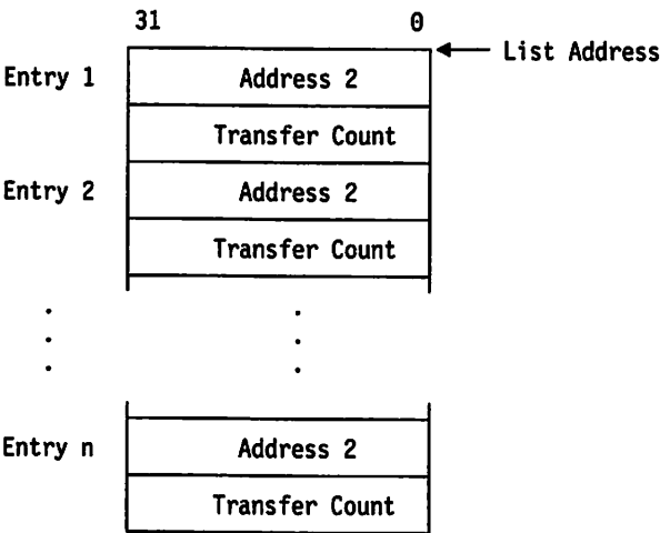
Figure 13. Indirect List Structure
