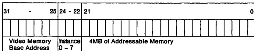
Figure 3-163. XGA Video Memory Base Address.
