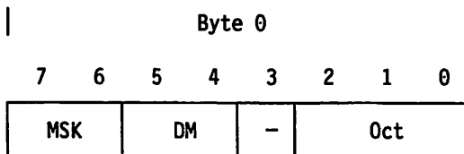
Figure 3-155. PEL Operations Register, Byte 0
