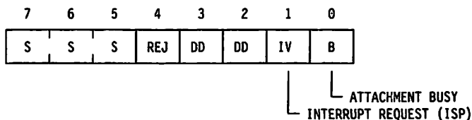
Figure 62. SCB Command Status Register
