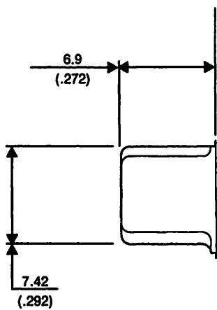
Figure 68. 60-Pin External Connector, Side View
