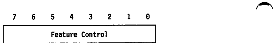
Figure 2-26. Feature Control Register, Hex 03DA/03BA and 03CA
