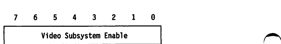
Figure 2-27. Video Subsystem Enable Register, Hex 03C3
