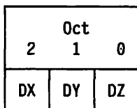
Figure 3-158. PEL Operations Register Direction Octant Values
