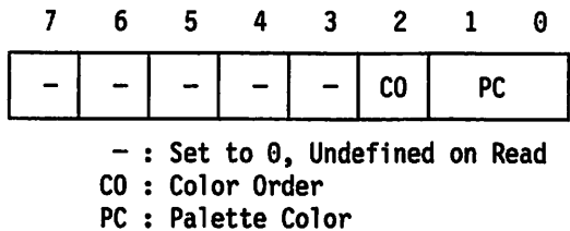
Figure 3-81. Palette Sequence Register, Index Hex 66
