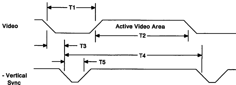
Figure 4-5. Vertical Timing, 400 Lines
