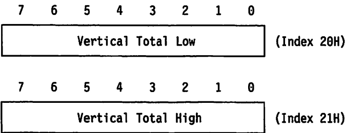
Figure 3-40. Vertical Total Registers, Indexes Hex 20 and 21
