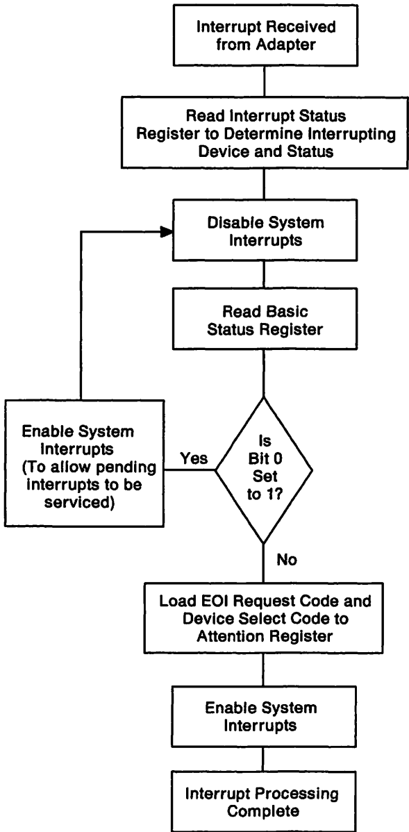
Figure 19. Processing an Interrupt
