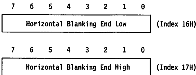
Figure 3-32. Horizontal Blanking End Registers, Indexes Hex 16 and 17
